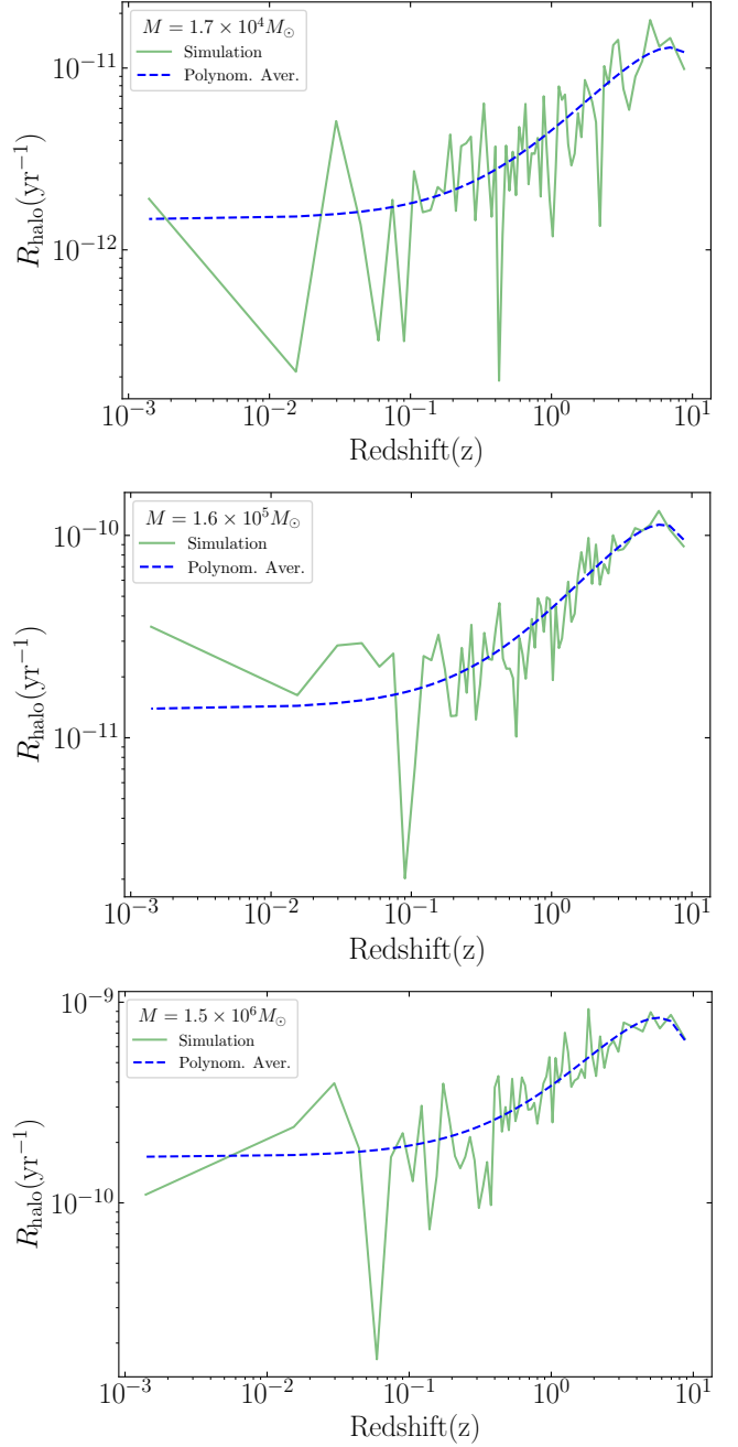
FIG. 14: As in Fig. 13, for a halo with mass M = 1.7 \times 10^4 M_\odot (top), M = 1.6 \times 10^5 M_\odot (middle) and M = 1.5 \times 10^6 M_\odot (bottom) at z = 0 . Two, three, and five spherical shells have been used for each halo, respectively.
