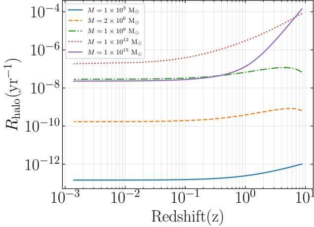
FIG. 15: Evolution of the merger rate per halo R_{\text{halo}}(z) , from the binary-single interactions. We show results for halos of different masses at z = 0 . The Ludlow16 concentration model has been used, incorporating a monochromatic PBH mass-distribution with M_{\text{PBH}} = 30 M_{\odot} .
