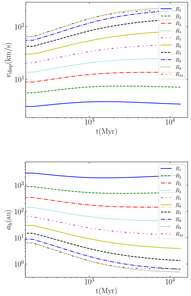
FIG. 11: The time evolution of the velocity dispersion v_{\text{disp}} (top panel) and a_h (bottom panel) for each of the ten spherical shells of a halo with M = 10^{12} M_{\odot} at the present era.
